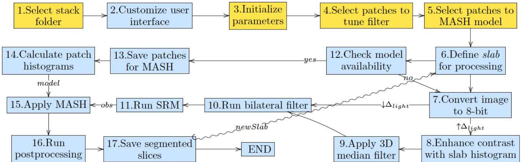
Figure 1: Flow diagram of Quant-CT segmentation workflow: yellow indicates user-interaction event and blue indicates a program action.
