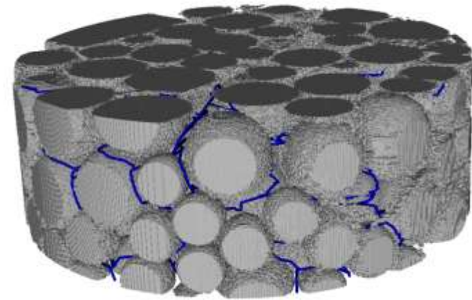
Pore network through porous material
