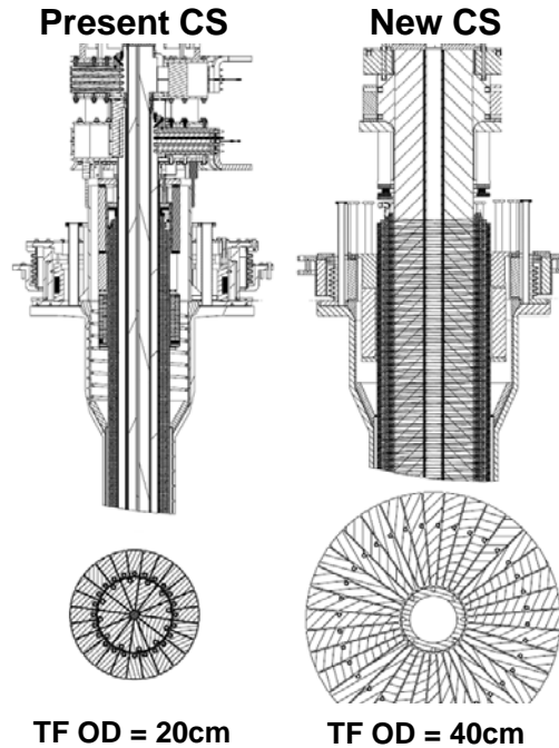
Center-stack magnets
