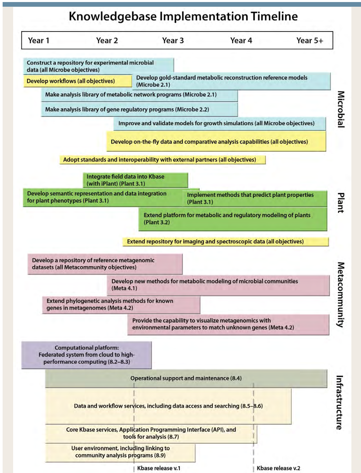
Fig. ES.6. High-Level Timeline for the Knowledgebase Implementation Plan. Light blue boxes represent tasks in the Microbial Science Area. Green boxes represent tasks in the Plant Science Area. Pink boxes represent tasks in the Metacommunity Science Area. Yellow boxes are tasks that apply to all objectives across all science areas. Infrastructure includes hardware (purple), operations (gray), and software (beige). Box height indicates relative level of effort for each task.
