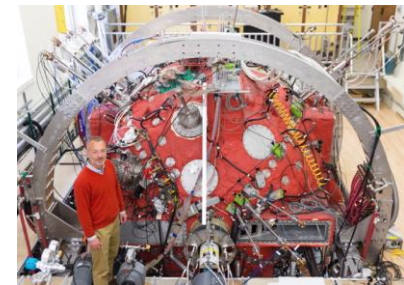
New WiPPL intermediate-scale experimental facility for general plasma science
