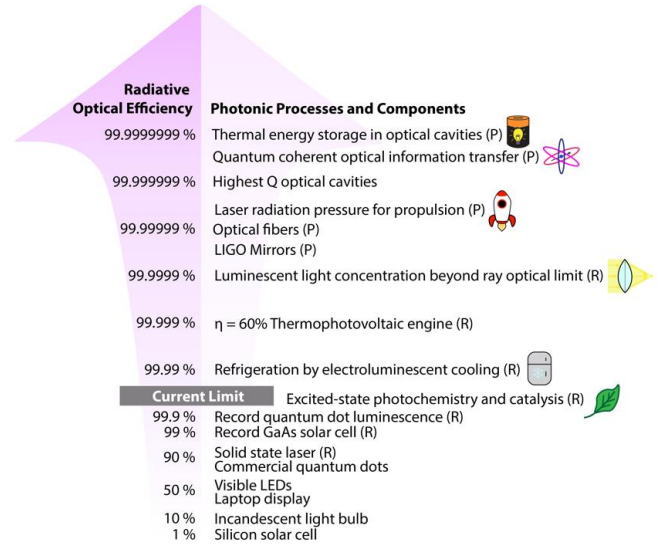
Figure 2: Passive (P) and Active radiative (R) systems that become possible with increasingly high optical efficiency.
