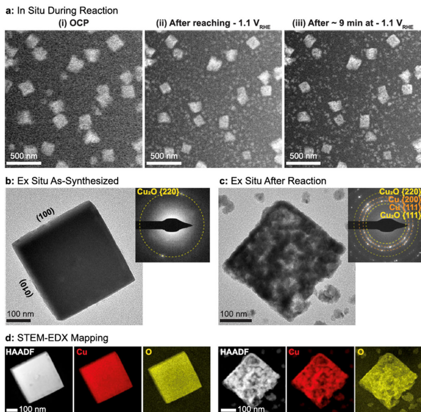
Figure 4-3. Morphology of \text{Cu}_2\text{O} cubes and their evolution during electrochemical reduction of \text{CO}_2 using ex situ TEM imaging and electron diffraction ( upper right inserts ) and STEM energy dispersive X-ray maps of the same cubes showing the copper and oxygen signals. Adapted with permission from P. Grosse et al., "Dynamic Transformation of Cubic Copper Catalysts during \text{CO}_2 Electroreduction and its Impact on Catalytic Selectivity," Nat. Commun. 12 (1), 1–11 under CC BY 4.0. © 2021.
