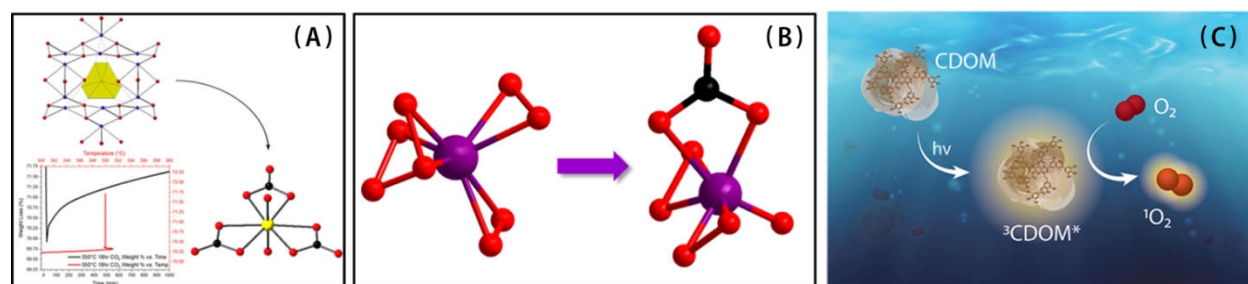
Figure 1-1. (A) Uranyl peroxide–superoxide conversion to uranyl carbonate via capture of \text{CO}_2 from air, and acceleration of the reaction with increased temperature. Adapted with permission from D. V. Kravchuk and T. Z. Frobes, ACS Mater. Au , 2 (1) 33–44 under CC BY 4.0. © 2022. (B) One step of conversion of tetraperoxovanadate to vanadyl diperoxide carbonate via capture of \text{CO}_2 from air in ambient conditions. Unpublished figure courtesy of May Nyman, Oregon State University. (C) Formation of reactive oxygen species via UV exposure of chromophoric dissolved organic matter (CDOM). Reprinted with permission from R. Ossola et al., “Singlet Oxygen Quantum Yields in Environmental Waters,” Chem. Rev. 121 (7), 4100–4146 under CC BY 4.0. © 2021.
