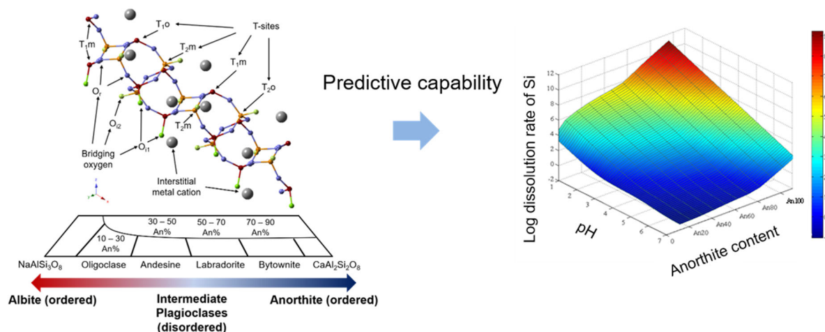
Figure 4-5. Plagioclase minerals are highly reactive aluminosilicates and are abundant in basalt as well as in minerals from deep saline aquifers. Fast dissolution of plagioclases can provide metal ions to form metal carbonate solids to store CO 2 . This image illustrates that the crystallographic information of these plagioclase minerals can be used to predict the dissolution rates of each mineral with varied anorthite contents at different pHs. Left , Reprinted with permission from Y. Yang et al., “A Mechanistic Understanding of Plagioclase Dissolution Based on Al Occupancy and T–O Bond Length,” Phys. Chem. Chem. Phys. 15, 18491–18501 © 2013 Royal Society of Chemistry. Permission conveyed through Copyright Clearance Center Inc. Right , Reprinted with permission from Y. Yang et al., “Effects of Al/Si Ordering on Feldspar Dissolution,” GCA 126, 595–613. © 2014 Elsevier.
