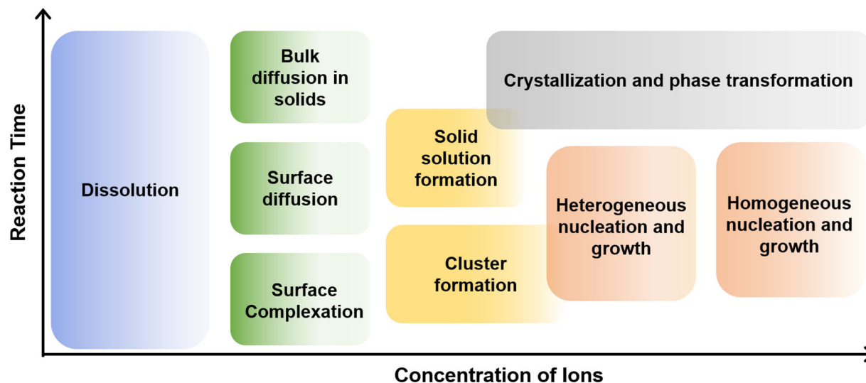
Figure 4-1. Dissolution, nucleation, precipitation, and phase transformation of minerals and materials at a wide range of time scales and concentrations (chemical potentials) of the systems. Unpublished figure courtesy of Young-Shin Jun, Washington University in St. Louis.
