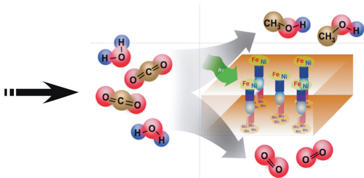
Artificial Photosynthesis
