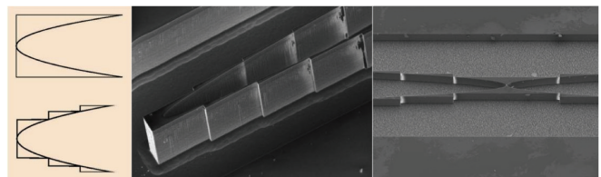
Left: A comparison of the solid refractive shape (top) with a kinoform shape (bottom). Middle: A parallel-to-point kinoform lens. Right: A point-to-point kinoform lens. ( Evans-Lutterodt et al., 2003 )
