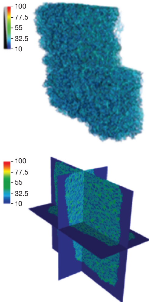
Figure 27 An ex situ neutron tomographic snapshot of the evolution (suspended) of lithium oxide loading of a carbon graphite foam battery electrode. Microstructural resolution is at the 50 \mu\text{m} size range.
