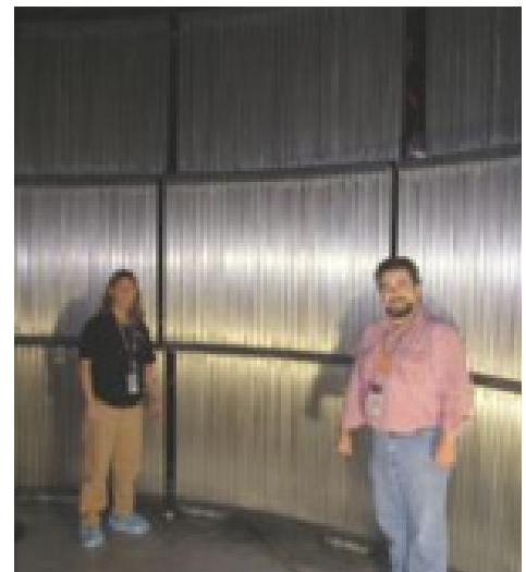
Figure 17 View of the large-area LPSD detectors at SNS Nanoscale-Ordered Materials Diffractometer (NOMAD) (left) and Wide Angular-Range Chopper Spectrometer (ARCS) (right) instruments.
