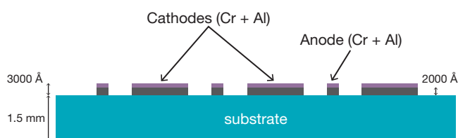
Figure 20 Cross-sectional view of micro-strip gas chamber (MSGC).
