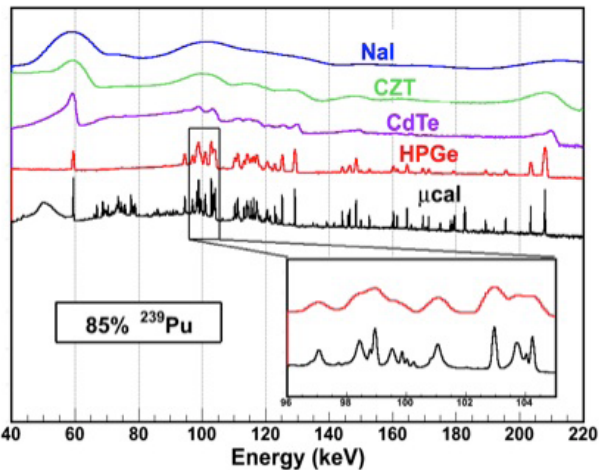
Figure 11 Comparison of scintillator (NaI), room-temperature semiconductor (CdTe), cryogenic semiconductor (Ge), and superconducting calorimeter energy resolution for very hard X-rays. Figure courtesy NIST/LANL.
