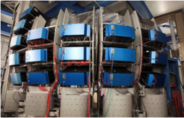
Figure 15 WLS fiber detector modules installed on POWGEN at the SNS.
