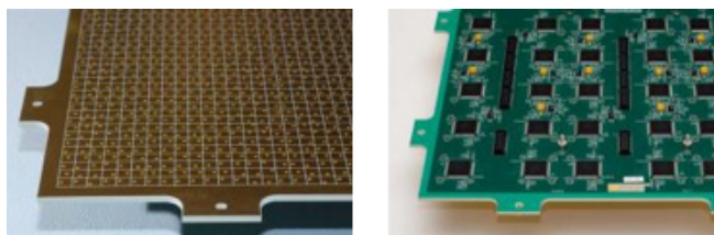
Figure 29 Sections of anode-pad board, showing independent 5 mm \times 5 mm pads (left) and ASICs on the underside of the board (right) to collect, measure, and digitize neutron signals.
