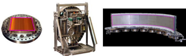
Figure 19 BNL detectors of the type shown left and center ( 20 \times 20 \text{ cm}^2 ) have been in operation for a number of years at the SNS magnetism and liquids reflectometers and at NIST. Advanced detectors of the type on the right ( 1.5 \text{ m} \times 20 \text{ cm} ) have recently been installed at LANSCE and the Australian Nuclear Science and Technology Organization (ANSTO).
