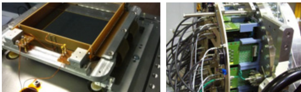
Figure 21 View of the MSGC and the MILAND detectors developed at ILL.
