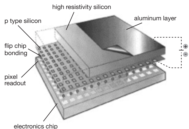
Figure 30 Hybrid pixel detector.
