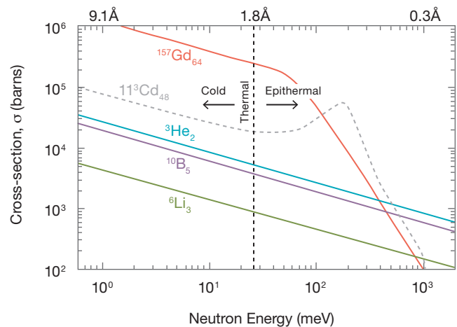
Figure 12 Neutron absorption cross section vs. neutron energy.
