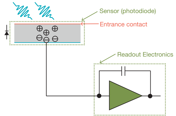
Figure 33 Connection of the sensor to its electronics.
