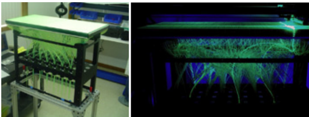
Figure 14 The WLS fiber detector, in daylight (left) and dark (right). The flat scintillator has an area of 77 × 38 cm 2 , and scintillation light is coupled by 308 and 152 fibers feeding 25 and 7 photomultipliers, respectively, for the X and Y axes.
