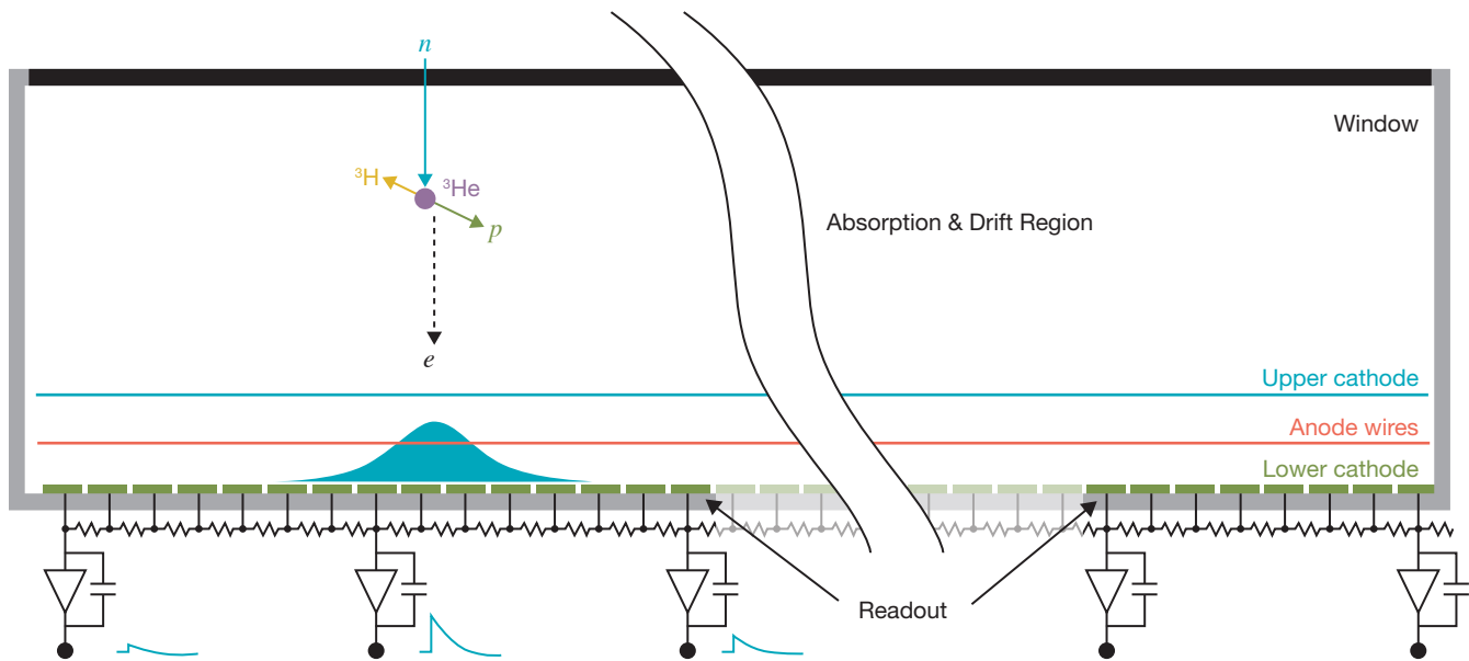
Figure 18 Schematic of advanced He-3 filled multiwire chamber.
