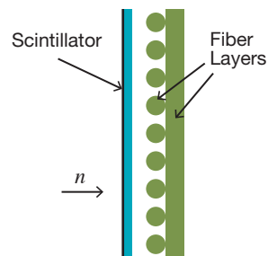
Figure 13 Cross section of WLS fiber detector, with crossed fibers placed to collect cone of scintillation light after neutron conversion in scintillator.
