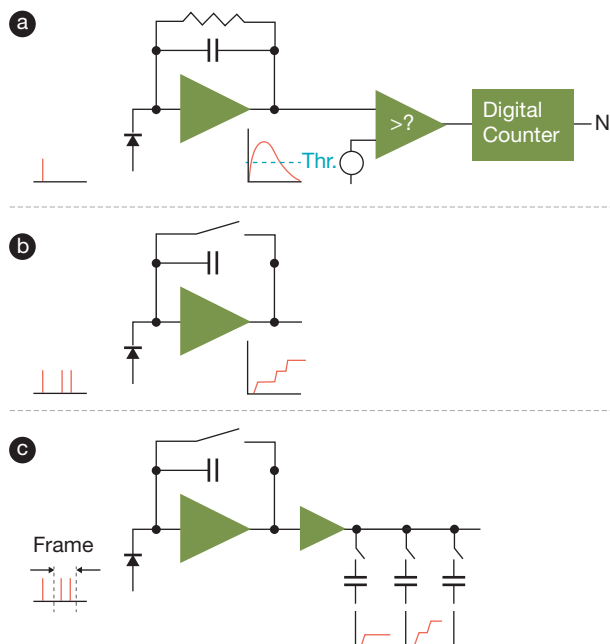
Figure 8 Different pixel architectures: (a) counting, (b) integrating, (c) fast-framing.
