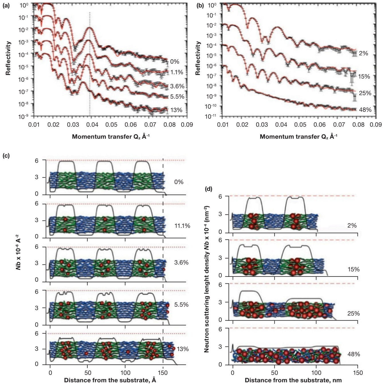
Figure 25 (a,b) Reflectivity profiles of symmetric (PS-d-b-PBMA) copolymer multilayers with different concentrations of small nanoparticles in (c) and big nanoparticles in (d). The volume fraction of nanoparticles is indicated in percent.
