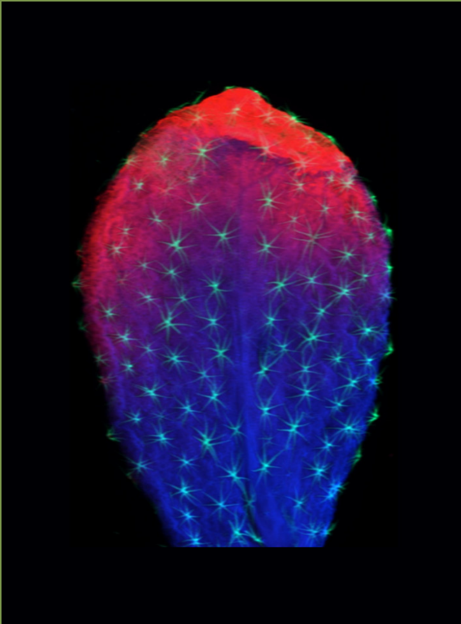
X-ray fluorescence microscopy image of a hydrated leaf from a cobalt hyperaccumulator plant ( Alyssum murale ), showing the elements cobalt (red), calcium (green), and potassium (blue). The image area is 4.22 mm x 7 mm, and has 420 x 700 pixels. The data was collected at a bending-magnet beamline (X27A) in only two hours.
