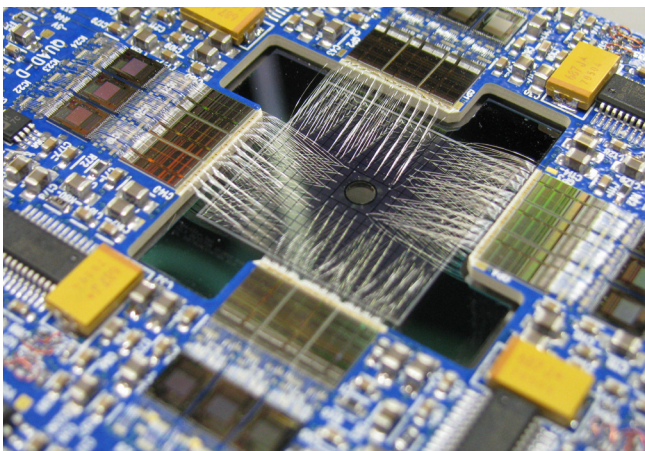
Figure 32 Maia detector showing intricate wire bonds.
