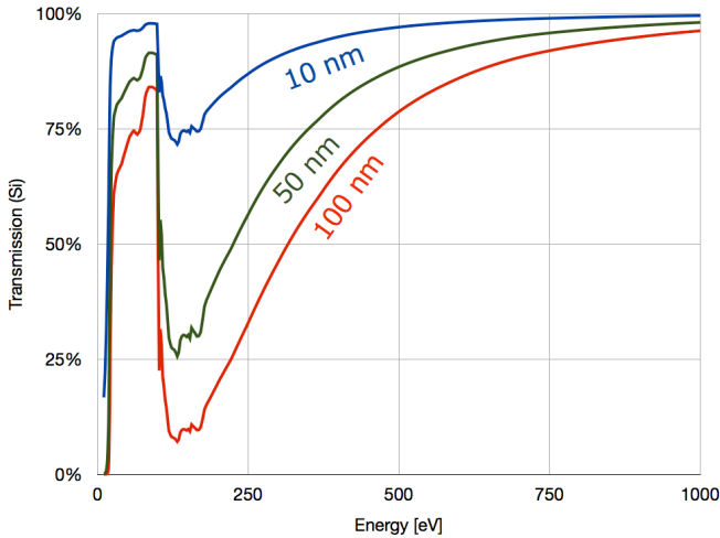
Figure 10 Transmission vs. energy for different thicknesses of entrance window.
