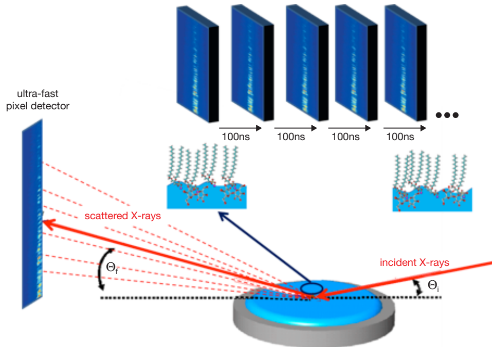
Figure 1 Photon correlation spectroscopy experiment.
