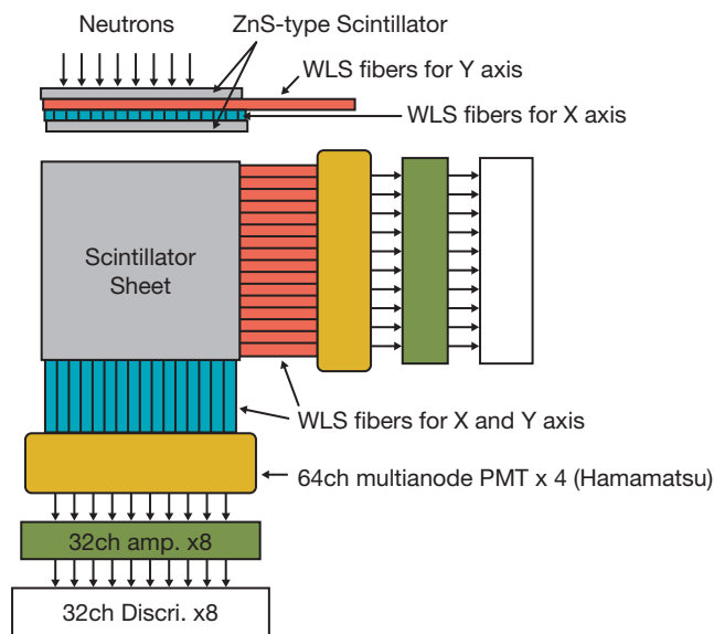
Figure 23 Key elements of the J-PARC scintillator detector.
