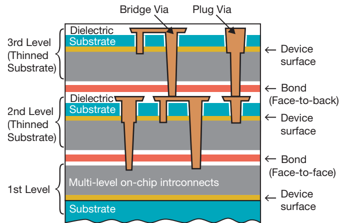
Figure 34 3-D interconnection.
