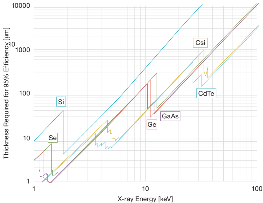
Figure 9 Thickness required for 95% X-ray efficiency as a function of X-ray energy for potential sensor materials.
