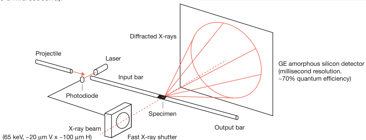
Figure 3 Studies of materials undergoing high strain rates generated by a Kolsky bar arrangement. The fast shutter is used to determine the temporal resolution of the experiment, as the detector is currently too slow and therefore the X-rays must be shuttered. The detector shown is what is currently available at the APS.
