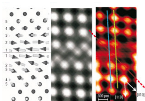
Figure 9 Atomic-resolution imaging of spin at a surface using scanning tunneling microscopy (Source: Bode et al., 2006, Nature Materials 5 477–481).
