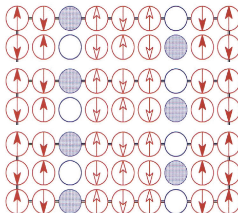
Figure 23 A schematic representation of a \text{CuO}_2 “stripe” indicating modulation in spin and charge
