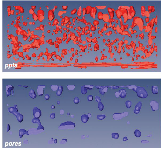
Figure 28 3-D reconstruction of the microstructure in a YBCO-coated conductor based on focused ion beam (FIB)-scanning electron microscopy (SEM) tomography. The total depth of the precipitates (ppts) and pores depicted here is \sim 1 \mu\text{m} (into the plane of the paper). (Courtesy of D. Miller, Argonne National Laboratory)
