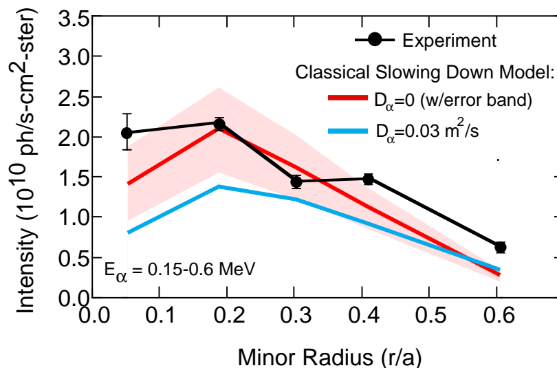
Fig. 2.10. Measured radial distribution of fusion \alpha particles compared with a classical slowing-down model prediction assuming no anomalous diffusion of \alpha particles ( D_{\alpha} = 0 ). Assumption of a very small rate of anomalous \alpha -particle transport is seen to be inconsistent with the data.
