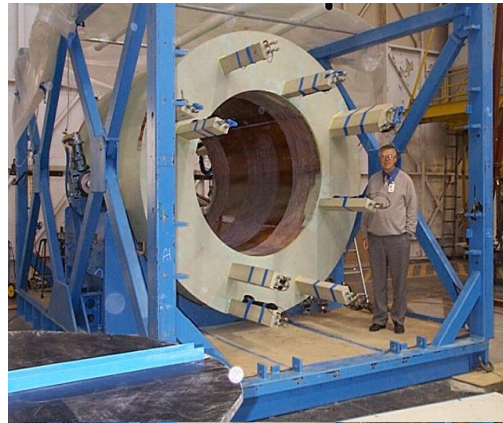
Fig. 2.24. Central solenoid model coil.
