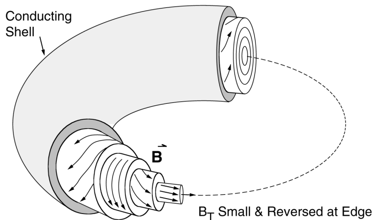
Fig. 2.16. Schematic of the magnetic field configuration in the RFP.
