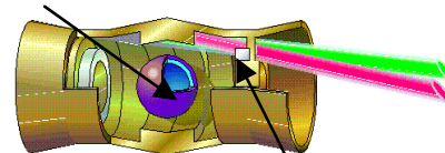
Heavy-ion beams heat X-ray converters inside hohlraum case (symmetric—one end shown).
