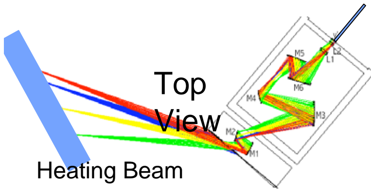
Motional Stark Effect
