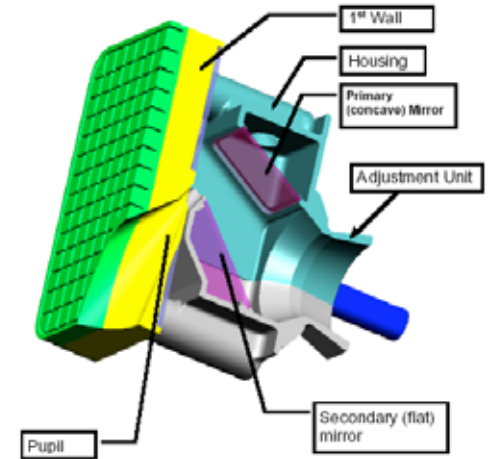
Visible/IR Cameras (upper)
