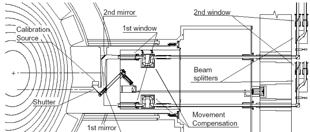
Electron Cyclotron Emission
