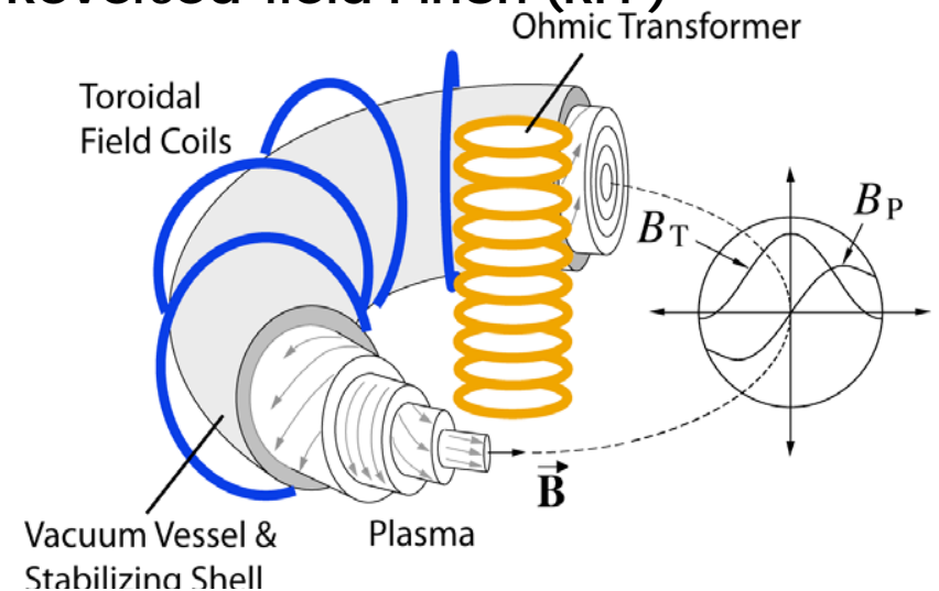
Reversed-field Pinch (RFP)
