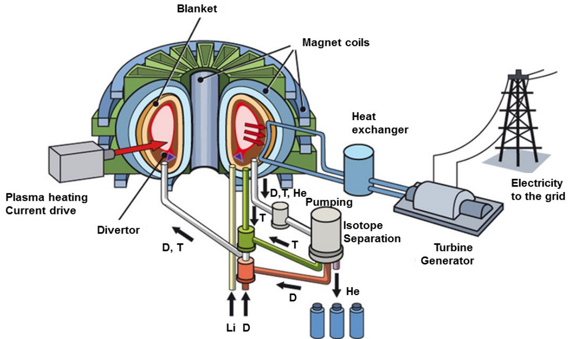
Layout of a future tokamak fusion power plant © IPP, http://www.ipp.mpg.de/14755/aufbau
