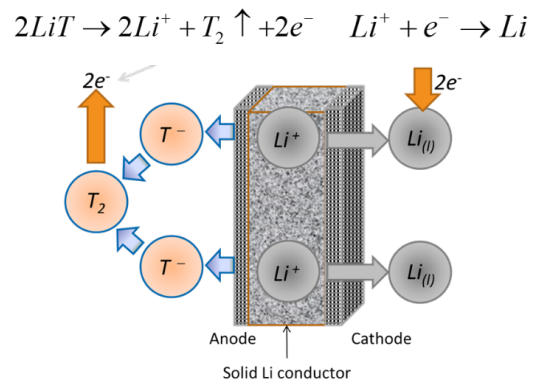
Figure 4.4.3: Schematic representation of a Lithium Conducting Electrolytic membrane 1 .
