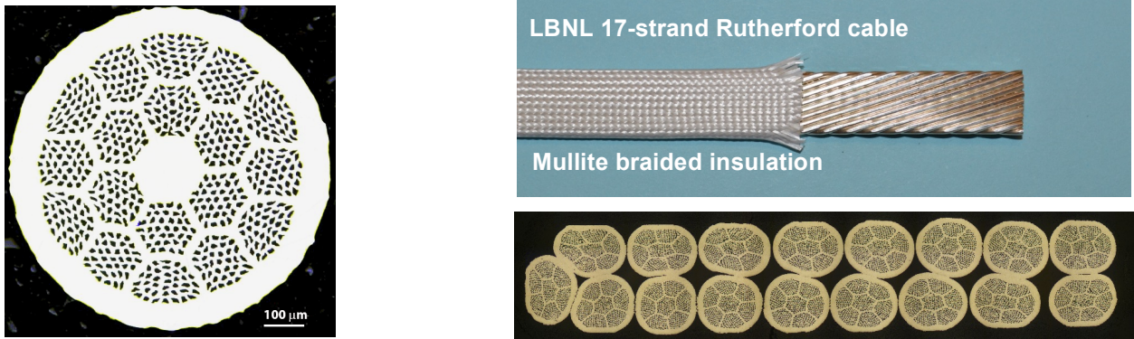
Figure 4.2.2. Bi-2212 strand cross section and Rutherford cable.
