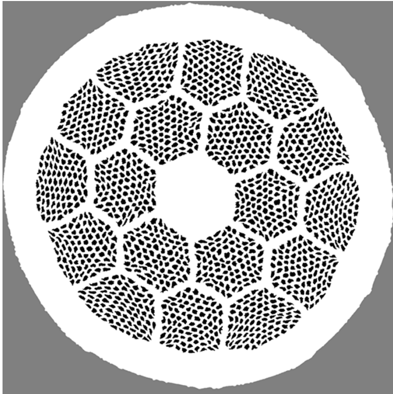
Bi-2212 strand cross section
