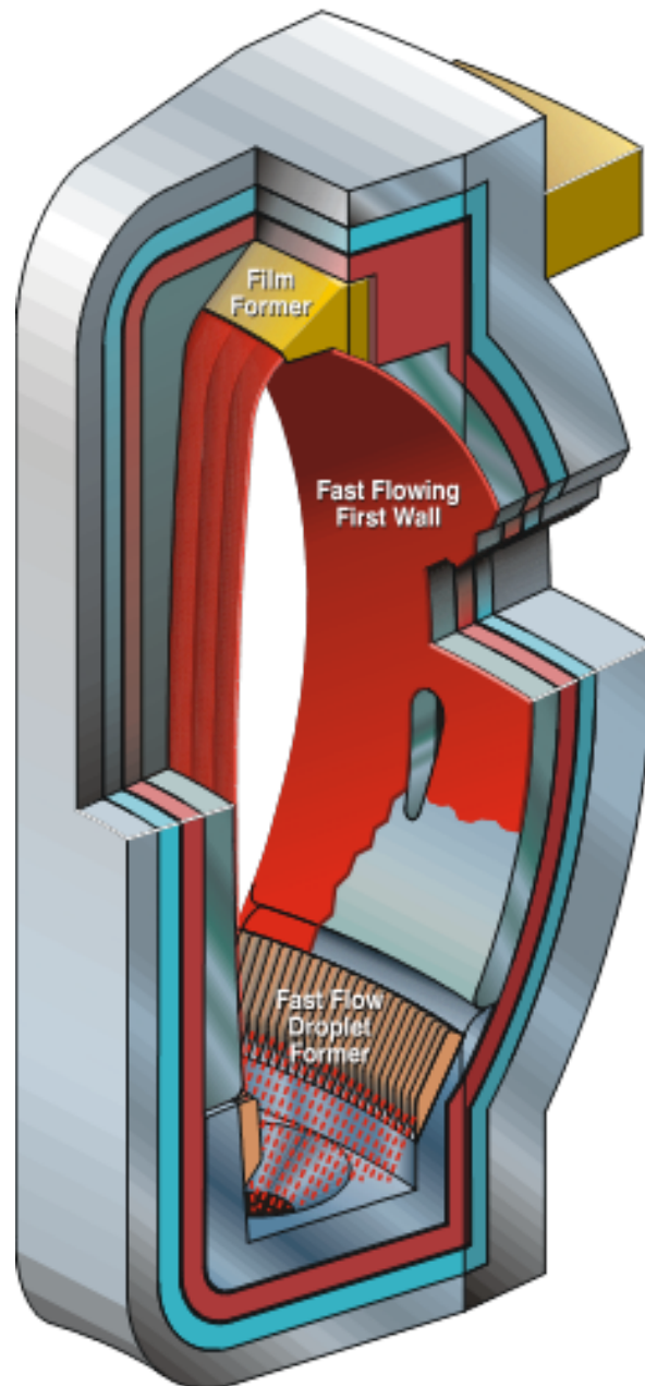
CLIFF Convective Liquid Flow Firstwall N.B. Morley et al. , http://slideplayer.com/slide/4939850/
