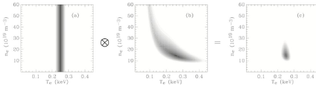
Figure 4.1.3. Probability Density Functions from a) soft X-ray data and b) Thomson scattering measurements of electron density, illustrating the combination of multiple diagnostics using a Bayesian statistical framework 9,10 . The result of combining a) and b) is the reduced posterior PDF (lower uncertainty) shown in c) for the combined data.
