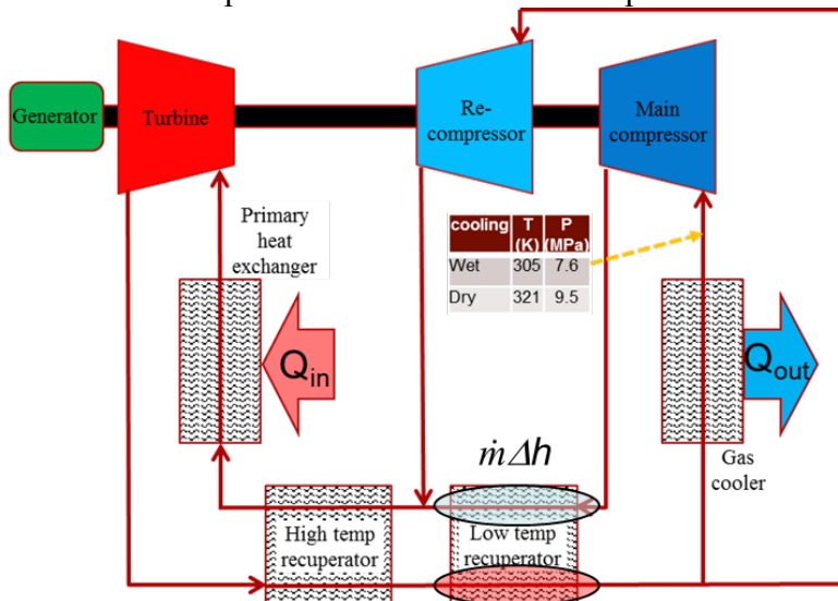
Figure 6.7.1. Supercritical CO 2 Recompression Closed Brayton Cycle diagram: the flow is split at points to optimize the thermal capacities of the heat-exchanging streams.
