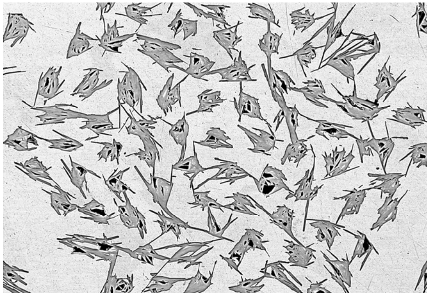
BSCCO Powder
