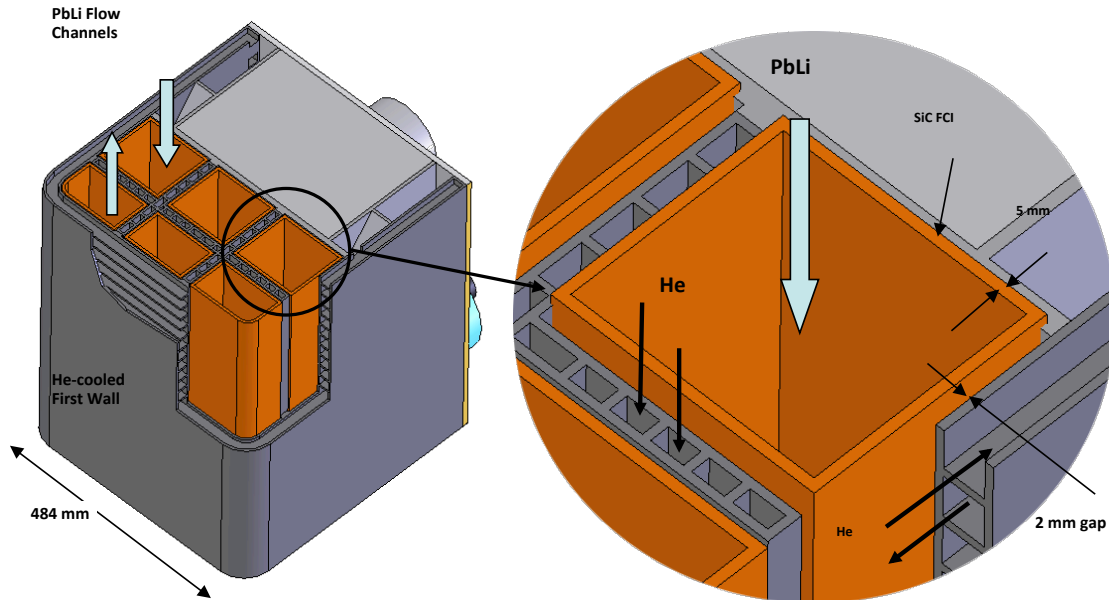
Figure 4.4.1: schematic representation of Dual Coolant Lead Lithium blanket
