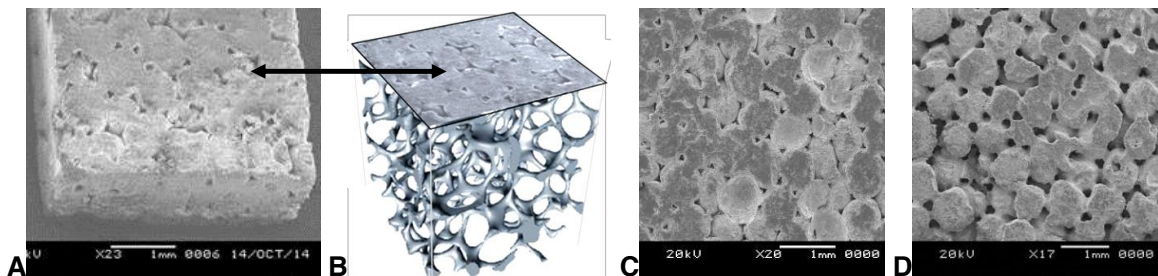
Figure 4.4.2A-D: SEM image of cellular breeder block (A), tomography scan showing network of interconnected internal micro-channels (B), and SEM images of 90% dense (C), and 78% dense (D) \text{Li}_2\text{ZrO}_3 cellular breeder fabricated using foam skeletons having different ligament diameters.
