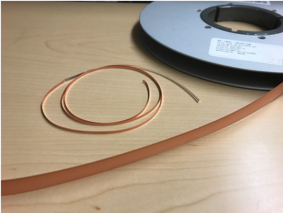
Figure 4.2.1. Two commercial tapes from SuperPower: 12 mm wide, 100 \mu\text{m} thick tape and 2 mm wide, 45 \mu\text{m} thick tape.
