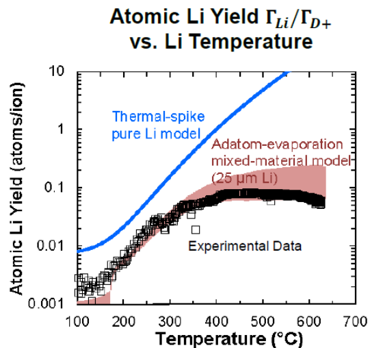
Figure 5.1. Erosion of lithium under high-flux deuterium bombardment as a function of surface temperature. The gross erosion, measured via spectroscopy, can be described with an adatom-evaporation and mixed Li-D material model that takes into account concentration-dependent hydrogen diffusivity in the bulk Li.
