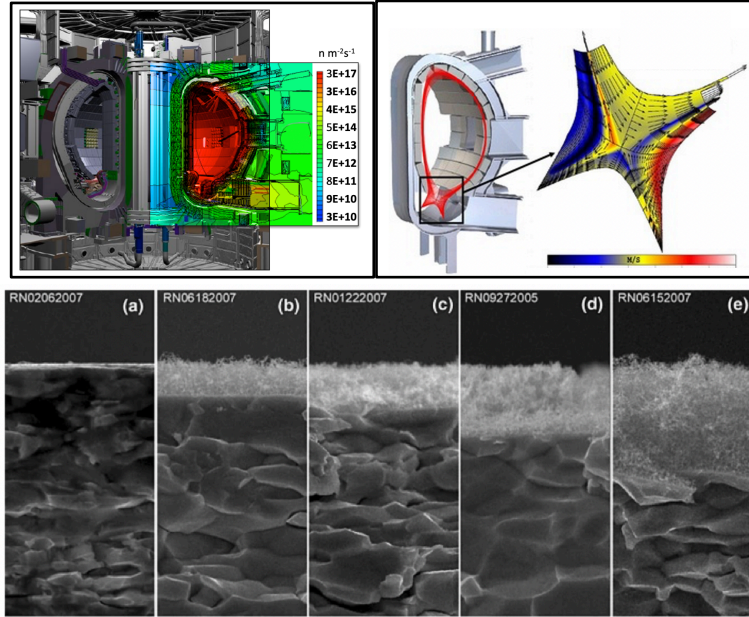
Figure IV.2-1: Resolution of materials/PMI issues will be critical to a successful fusion reactor. (Top left) Expected neutron load in the different ITER chamber and structural components. (Top right) Contour plot of the particle flux in the divertor region. (Bottom) Sequence of SEM images showing the degradation of a W surface through the development of ‘fuzz’ structures.
