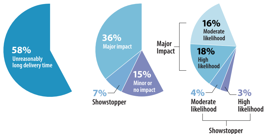
Fig. 2.5. Overview of the impact and likelihood of procurement issues caused by unreasonably long delivery times.
