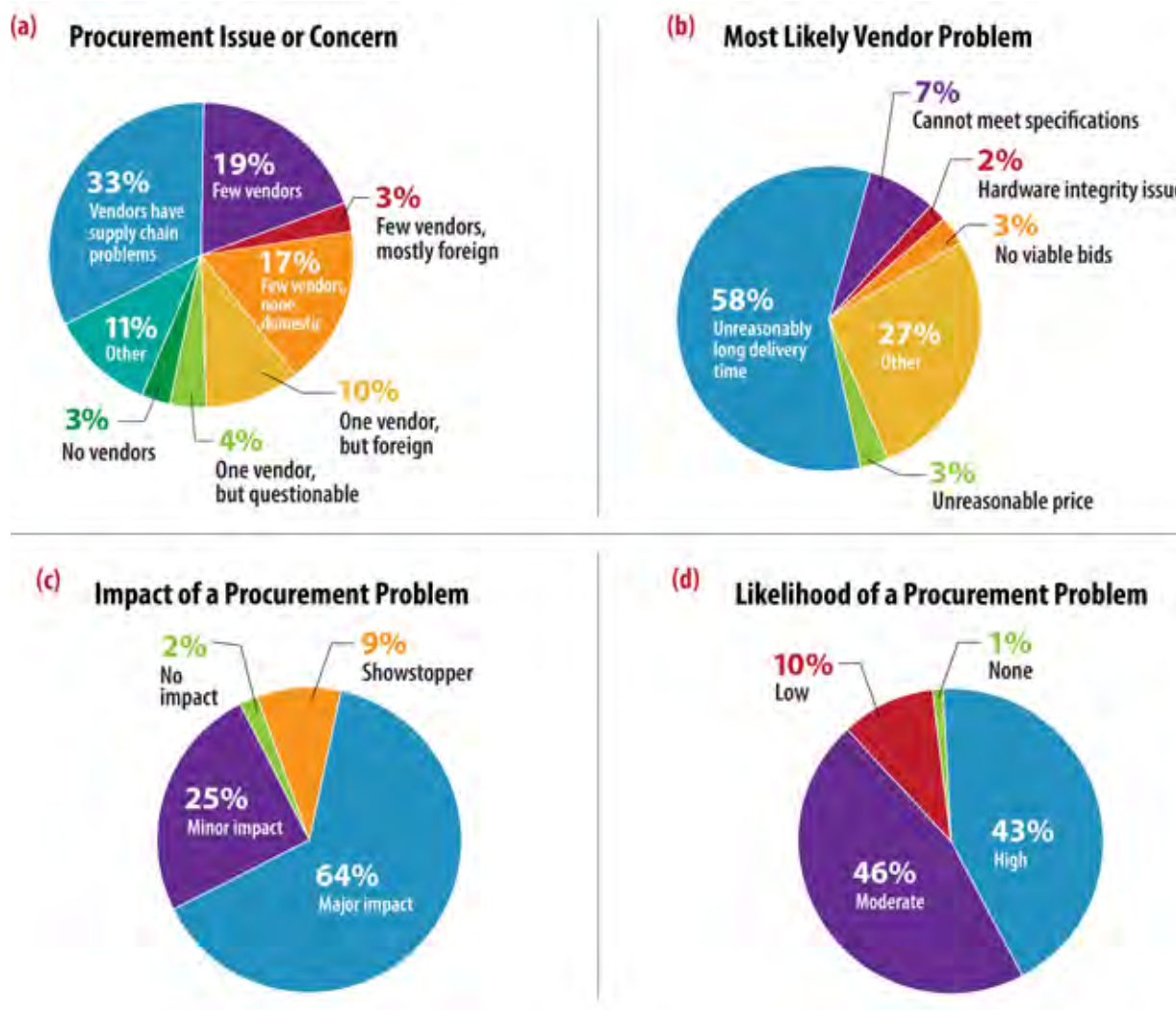
Fig. 2.4. Summary of the approximately 180 components identified as experiencing procurement challenges. Graphics show (a) the procurement issue or concern, (b) most likely vendor problem, and (c, d) impact and likelihood of the procurement problem.
