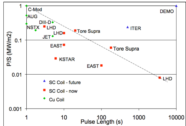
Fig 4.2 Development and Integration of Long Pulse Plasma Wall Solutions
